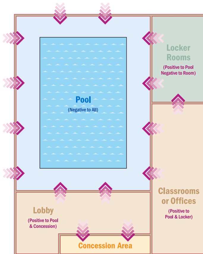
Figure 6. Building pressurization
