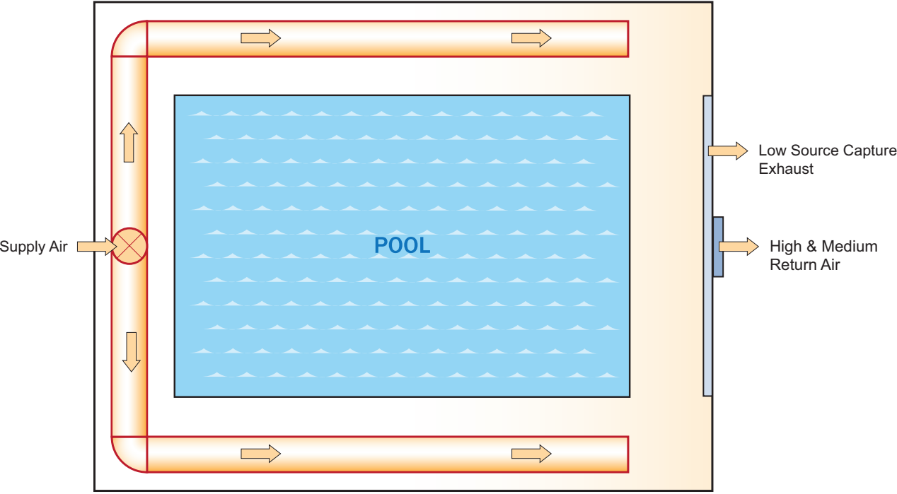
Figure 8. Top view of duct design
