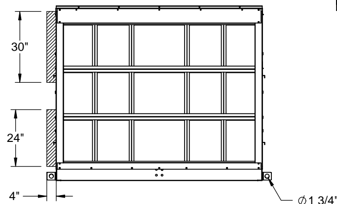
DUCT CONNECTION w/DAMPER OPTION SHOWN
