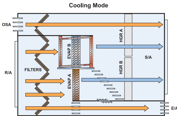
Figure 4 - Dehumidification in Cooling Mode
