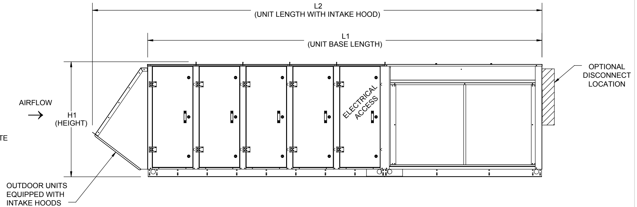
ACCESS SIDE VIEW (2, 6, 7)
