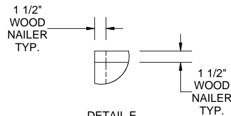
DETAIL E SCALE 1 : 12
