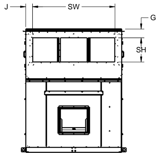
HOODS OMITTED FOR CLARITY
