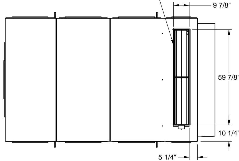
DUCT CONNECTION w/ DAMPER OPTION SHOWN
