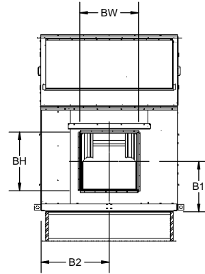
SECTION A-A END OF UNIT
