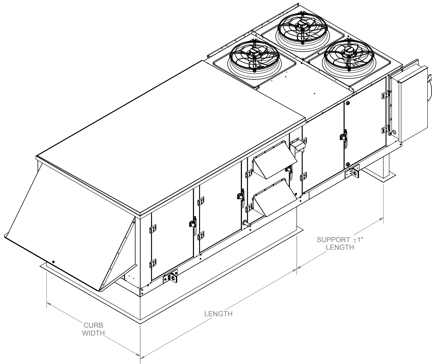
TWO PIECE CURB DETAIL
