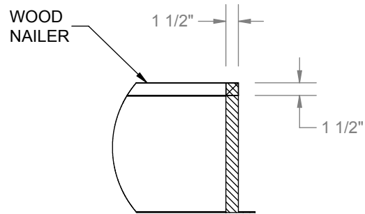
DETAIL C SCALE 1 : 16
