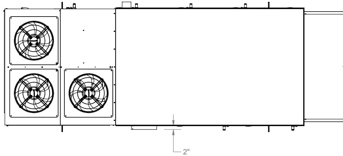
TOP VIEW LEFT DISCHARGE CONNECTION
