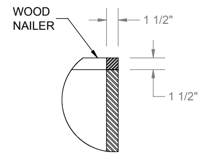
DETAIL G SCALE 1 : 12
