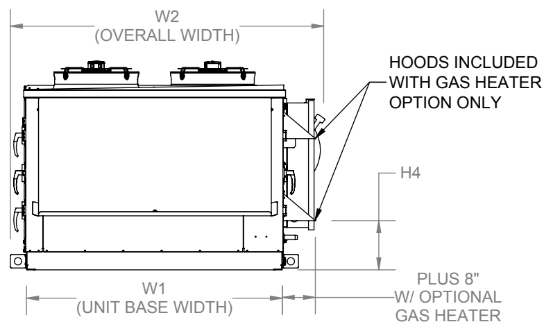
OUTDOOR AIR INTAKE VIEW 5 4
