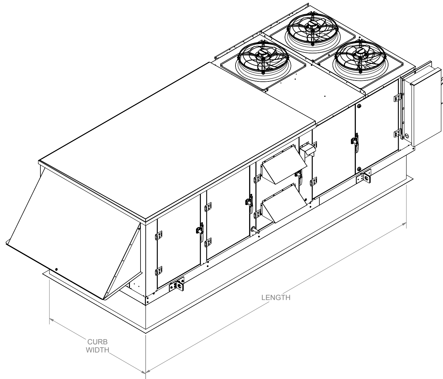
ONE PIECE CURB DETAIL
