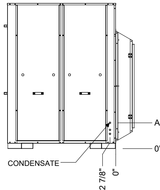
LEFT CONDENSATE OPTION LEFT SIDE VIEW
