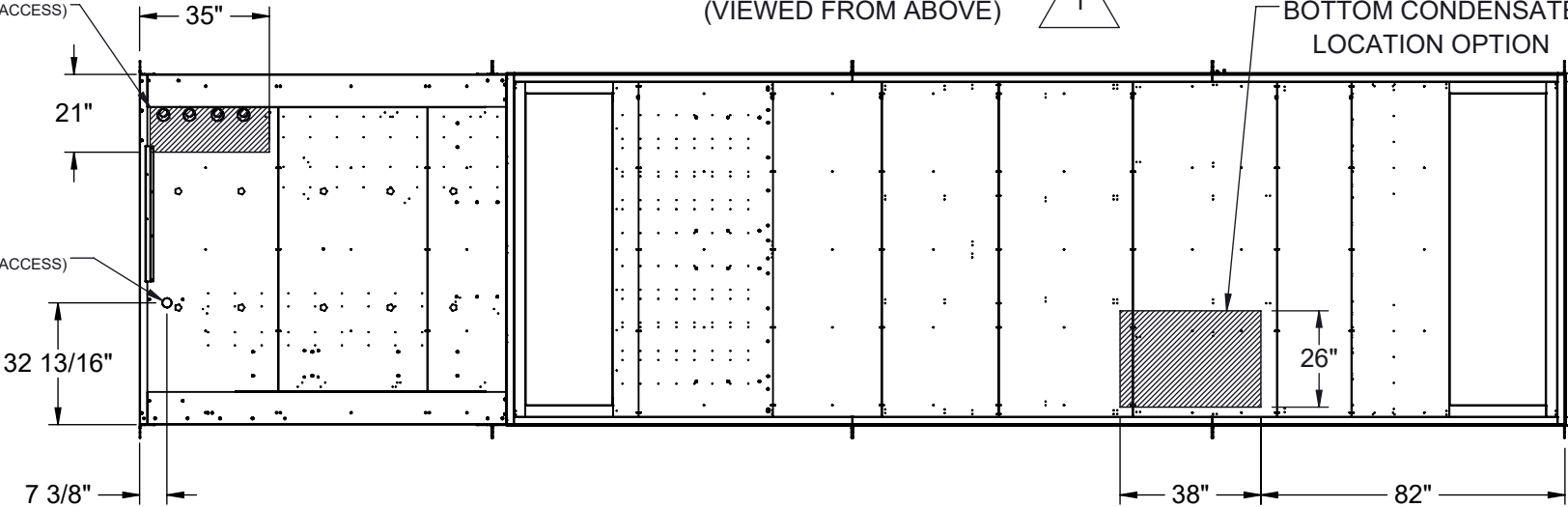
BOTTOM CUSTOMER CONNECTIONS (LEFT HAND ACCESS SHOWN) (VIEWED FROM ABOVE)
