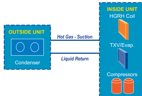
Figure 4 - VerticalAire™ Line Set Schematic
