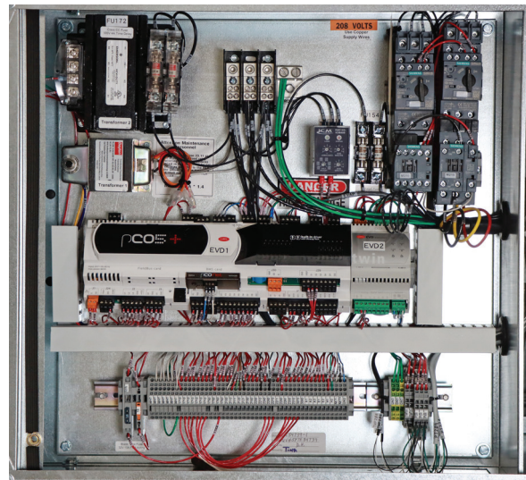
Figure 5 - VerticalAire™ Electrical Panel Detail
