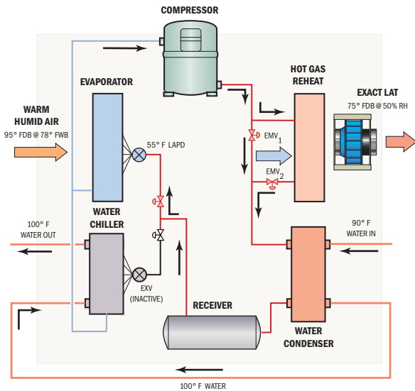
Figure 2 - Q-Pump Schematic with LAT Control: Cooling Mode
