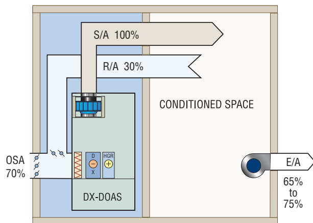
Figure 3 - DOAS CO 2 Control
