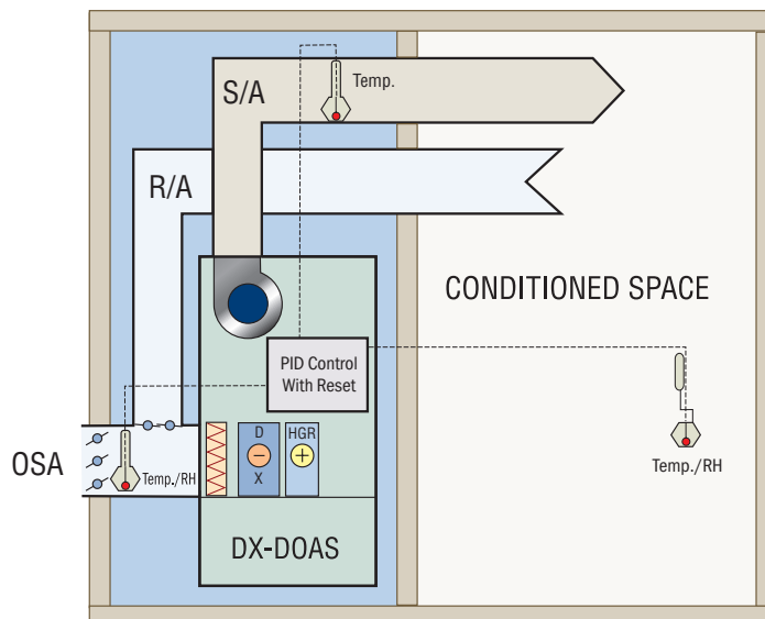
Figure 1 - Zone Reset Control Configuration
