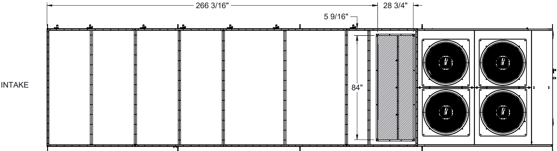
TOP SUPPLY OPTION (TOP VIEW) (LEFT HAND ACCESS SHOWN) (NO ORIENTATION CHANGE FOR RH OR LH ACCESS)
