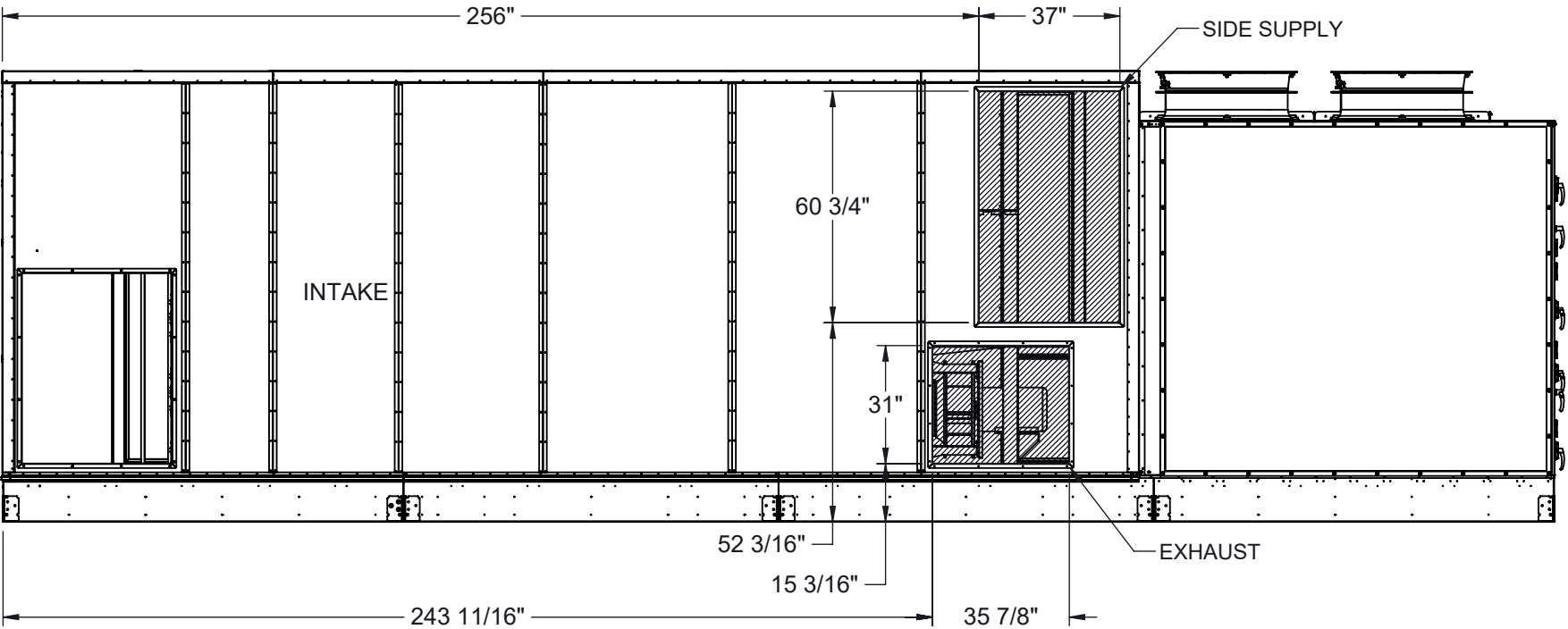
SIDE SUPPLY OPTION (RIGHT SIDE VIEW)
