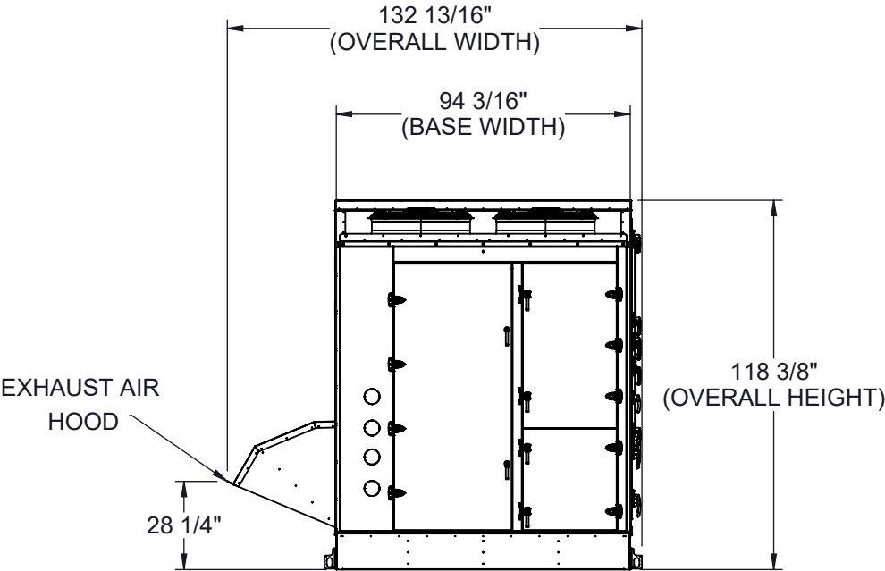
BACK VIEW
